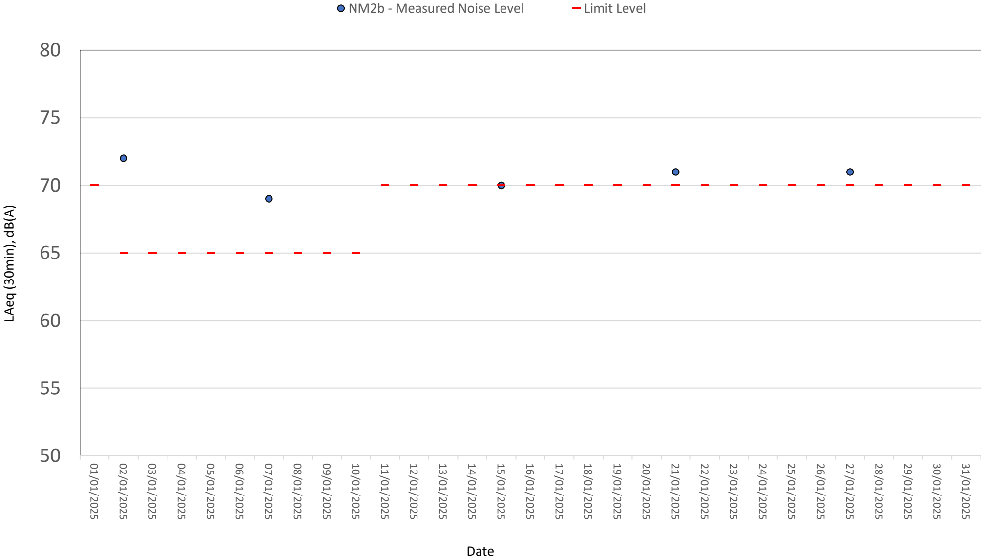
Normal Weekdays Noise Monitoring Results at NM2b(Leq, 30min)
